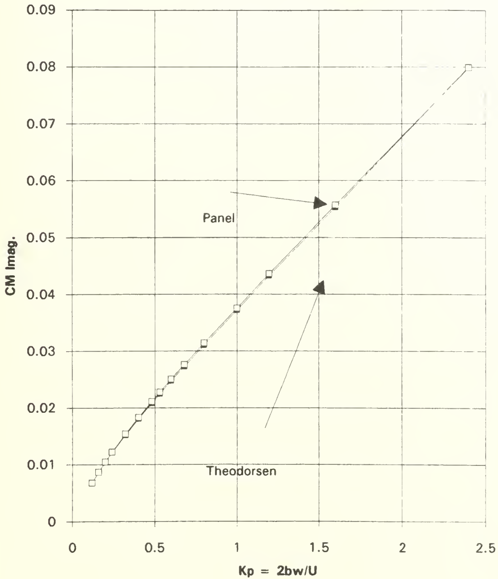
Imag. Part of CM for Panel and Theodorsen (plunge, .0833 h/2b, .37c, NACA0007,75 panels top and bottom, 3cycles of 65 calculations)
